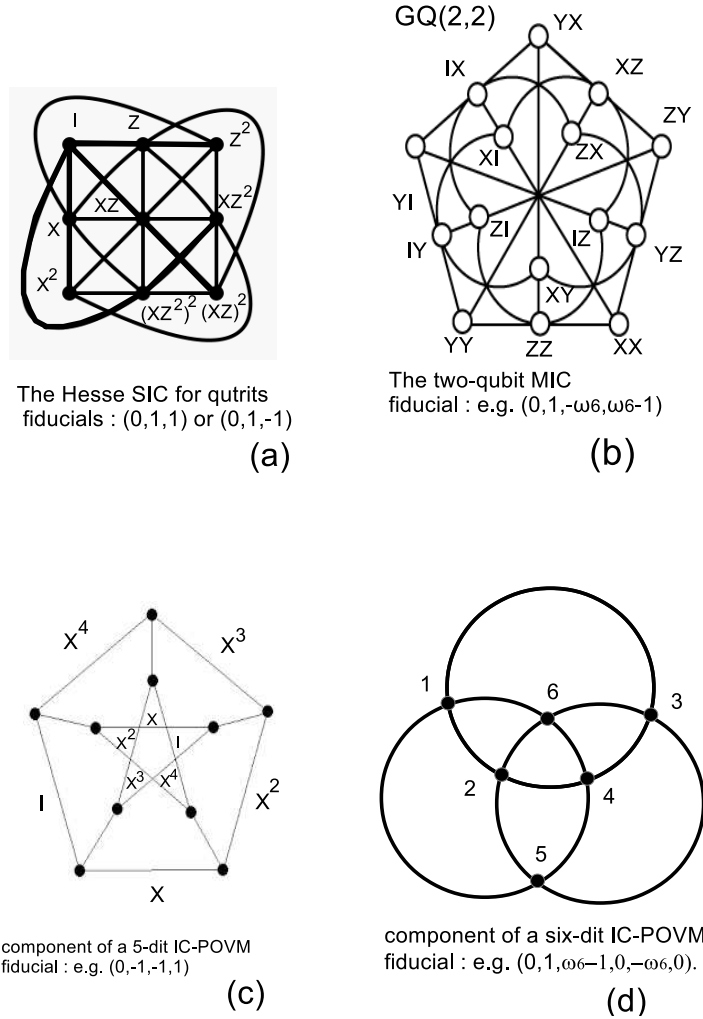
FIGURE 1. Geometrical structure of low dimensional MICs: (a) the qutrit Hesse SIC, (b) the two-qubit MIC that is the generalized quadrangle of order two GQ(2, 2) , (c) the basic component of the 5-dit MIC that is the Petersen graph. The coordinates on each diagram are the d -dimensional Pauli operators that act on the fiducial state, as shown. For the 6-dit case in (d), the coordinates are made explicit in the caption of [8, Fig. 4].
